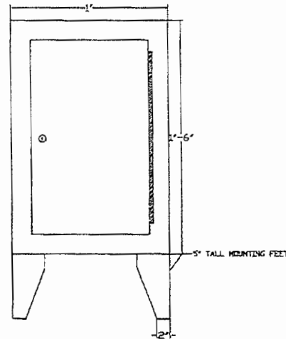
GROUND MOUNT RECEPTACLE CABINET
